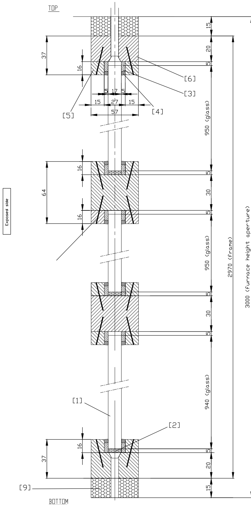
Pyrobel 16 in a timber frame SECTION D-D
