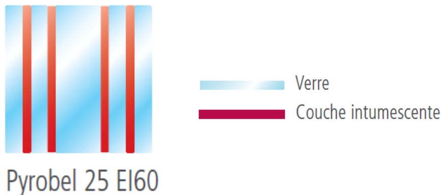
Figure 1 : Structure d’un Pyrobel 25 Stock-Size
